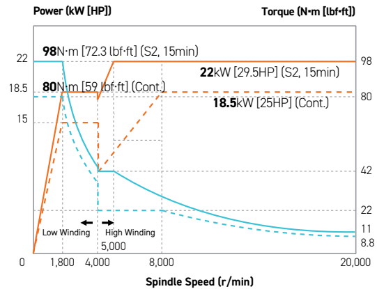
Built-in 20,000rpm
